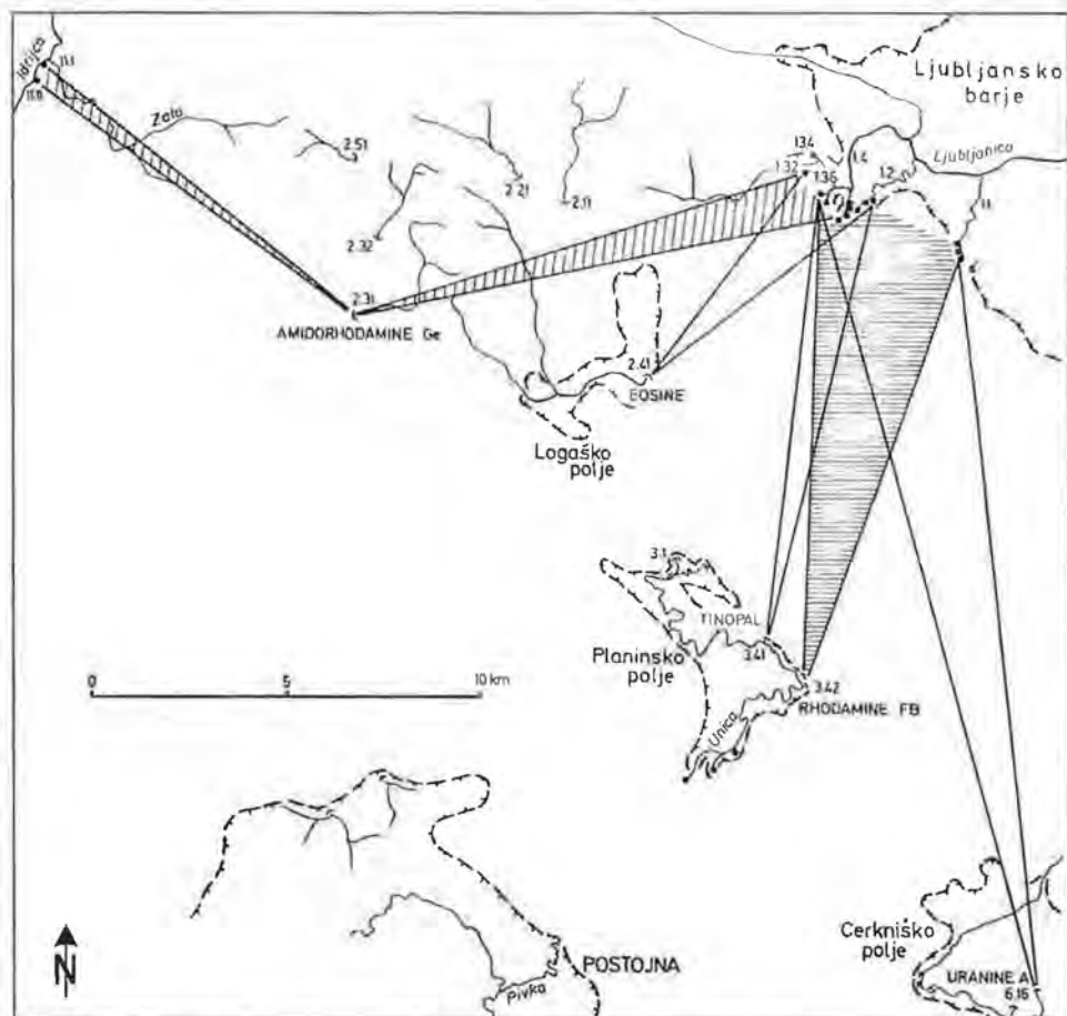
Fig. 2.2: Distribution of the fluorescent tracers in the Ljubljana catchment area in the comparative tracer experiment 1975 (from R. GOSPODARIĆ & P. HABIČ, 1976).
