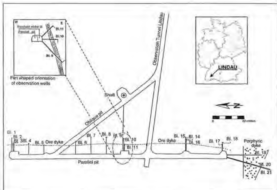
Fig. 3.4: Plan of the Lindau fractured rock test site showing the injection borehole Bl. 8 and the observation borehole Bl. 10.
