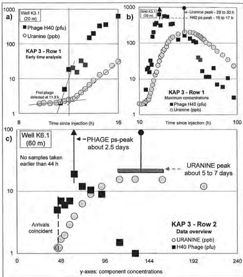
Fig. 4.8: Tracer test KAP 3 concentration history. a) well K3.1 early time analysis, b) well K3.1 maximum concentrations, c) well K6.1 data overview.
