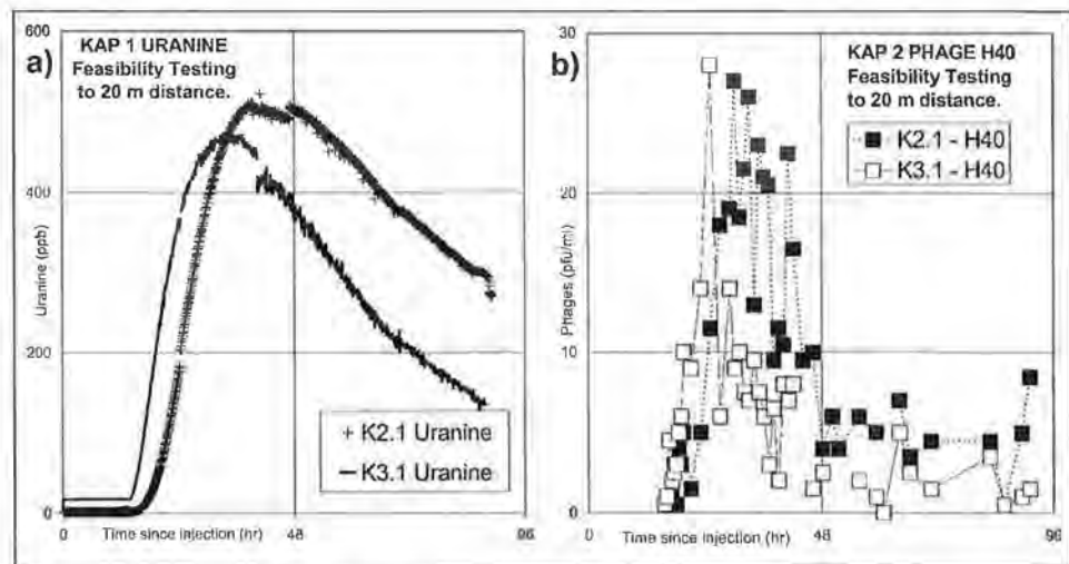
Fig. 4.7: Tracer tests KAP 1 and KAP 2 concentration history at wells K2.1 and 3.1. a) KAP 1 (uranine), b) KAP 2 (phage H40).
