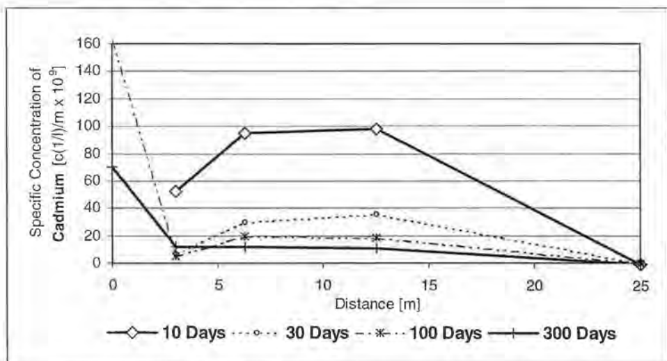
Fig. 4.24: Longitudinal profile (0–25 m) for cadmium. Observation times and specific concentration in Y-axis (left) as shown in fig. 4.23.
