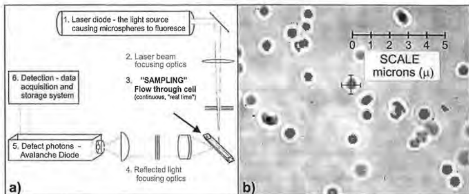
Fig. 4.12: Microspheres. a) instrumentation basis components, b) latex microspheres photomicrograph (after S. NIEHREN, 1998).
